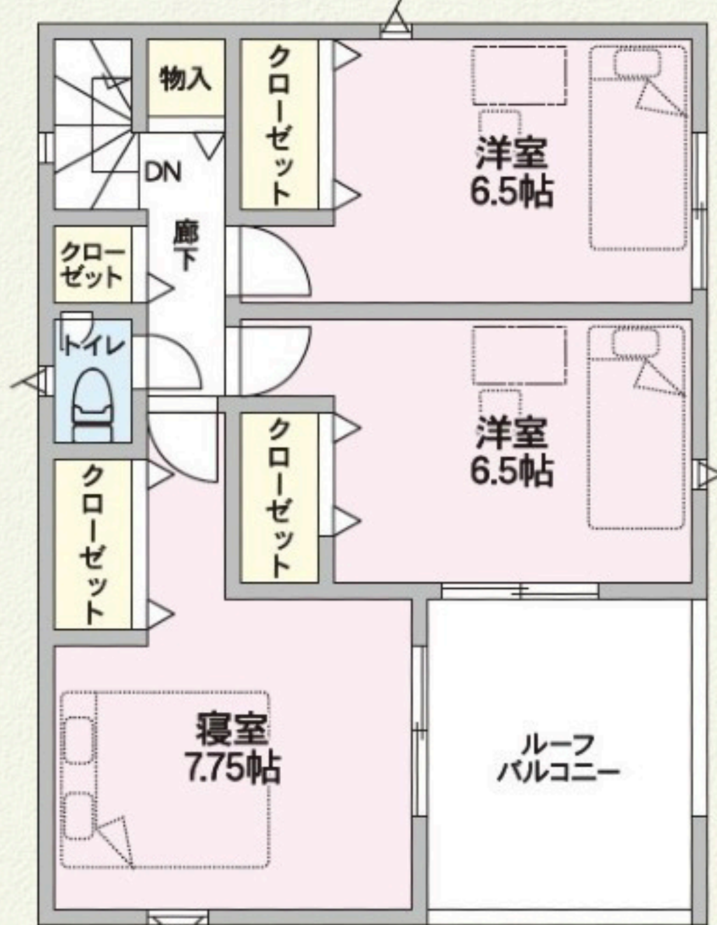
2F 45.35m 2
